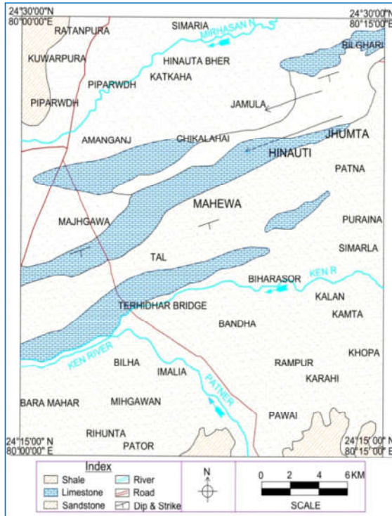
Fig. 1.2 Geological Map of the Study Area
