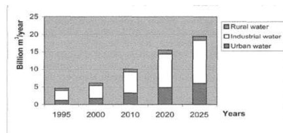
Fig. 2 : Trend of water consumption demand in Tons River
