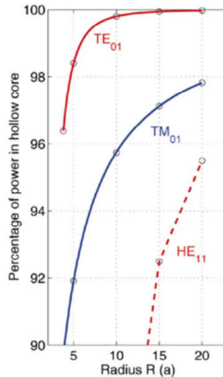
Fig. 1 : The figure shows that TE 01 mode has the largest captivity for all values of R and proceeds to 100% at a higher rate than the other modes that establishes its characteristics.
